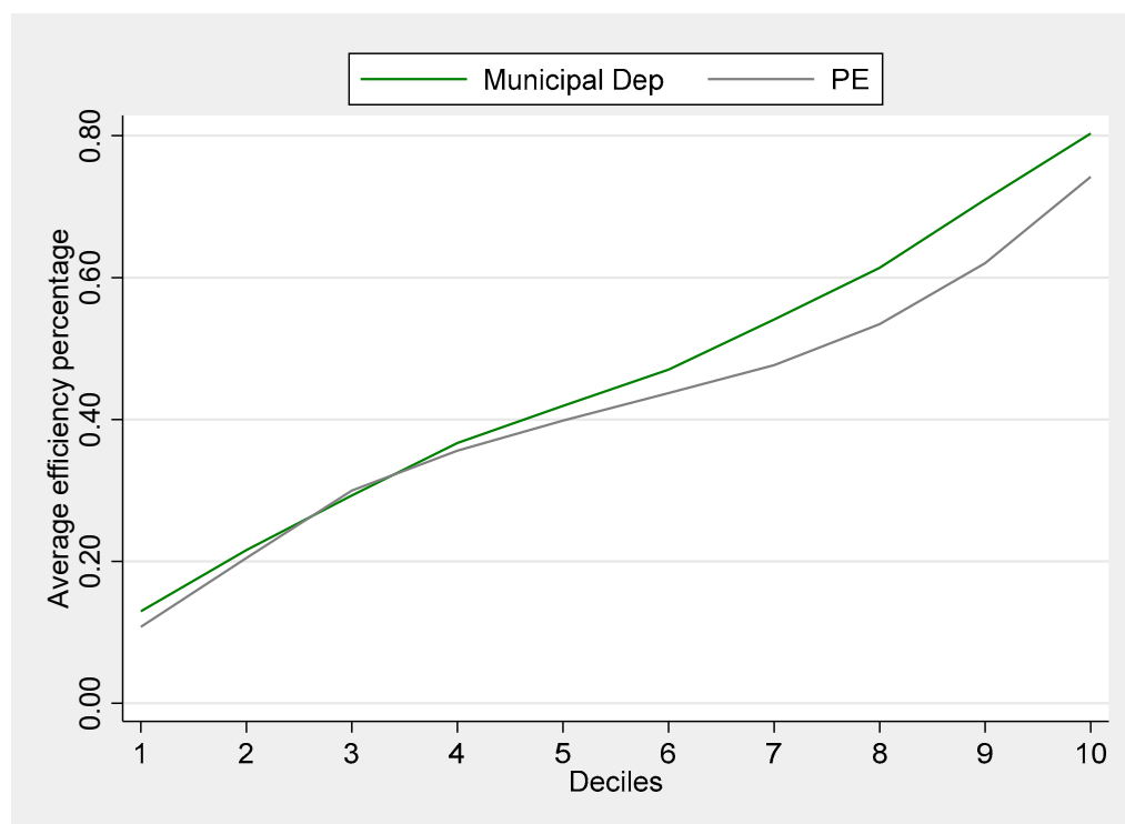
Figure 4. Bias-corrected technical efficiency deciles by management type.
