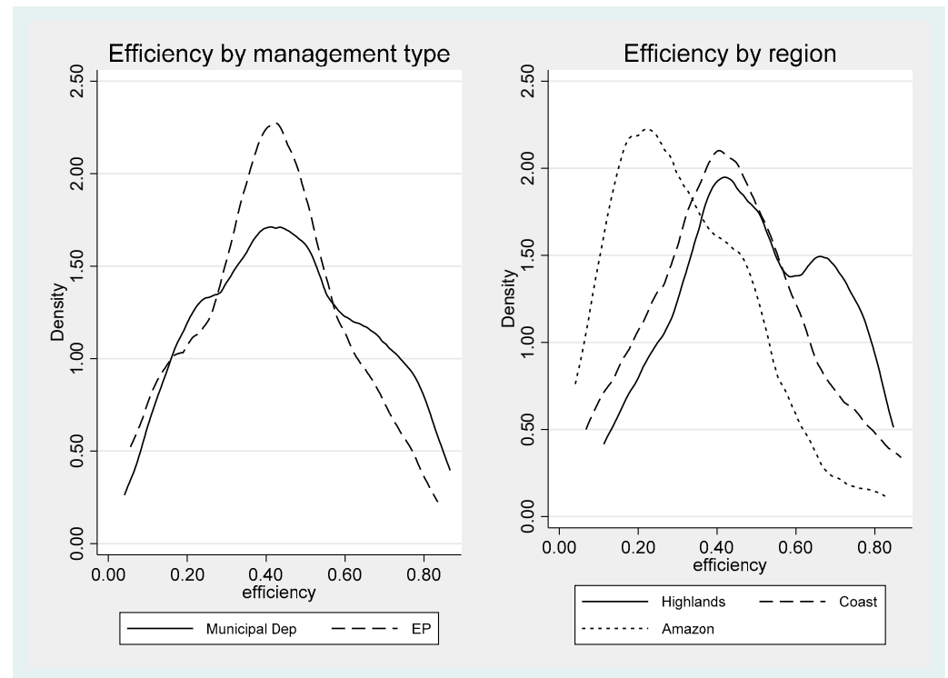
Figure 3. Distribution of technical efficiency with bias correction, by type of management and region.
