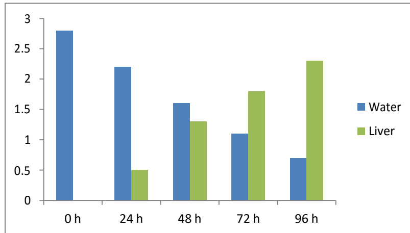
Fig. 1. Residue of deltamethrin in water and liver tissue as determined by High performance liquid chromatography (HPLC), 6 \mu g/L of deltamethrin was added initially.
