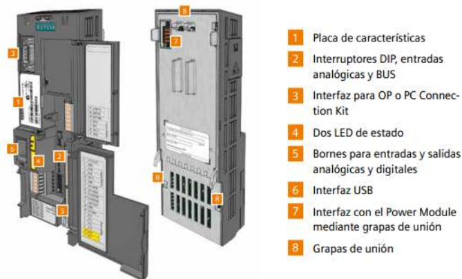
FIG.19 Control Unit 25
