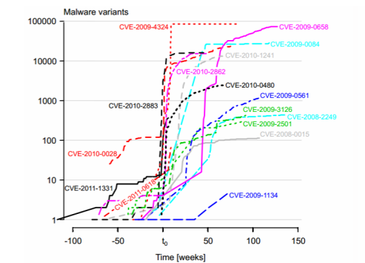
Figure 6: Number of exploit variations before and after the CVE disclosure. t0 is the disclosure date [16].
