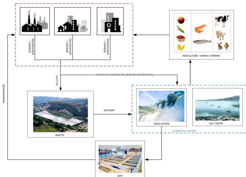
Figure 1. Description of the origin and transport of ECs in water.
