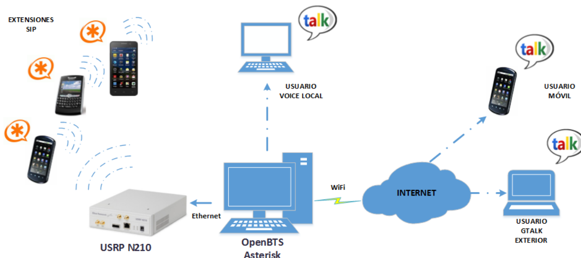
Figura 5. Diagrama de red OpenBTS-Asterisk-GoogleTalk.
