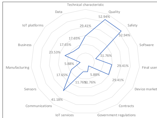
Fig. 2. Analyzed criteria trends to IoT device selection.
