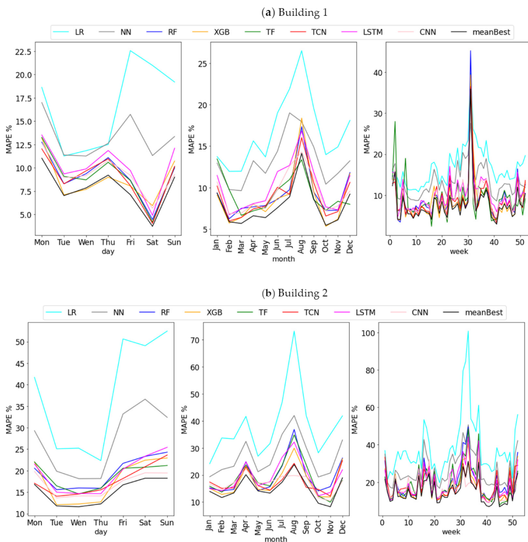
Figure 6. (a) Performance of forecasting models by day, month, and week in building 1; (b) performance of forecasting models by day, month, and week in building 2.
