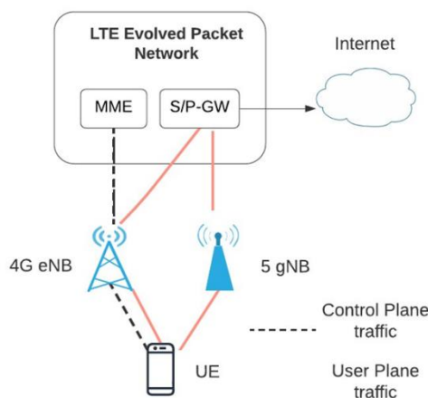
Figure 5: Non-standalone architecture.
