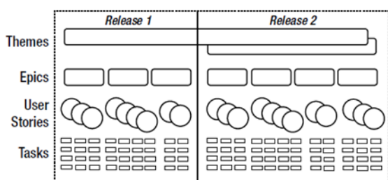
Figure 2. Hierarchy of requirements types within an Agile context (taken from (Moreira 2013)).
