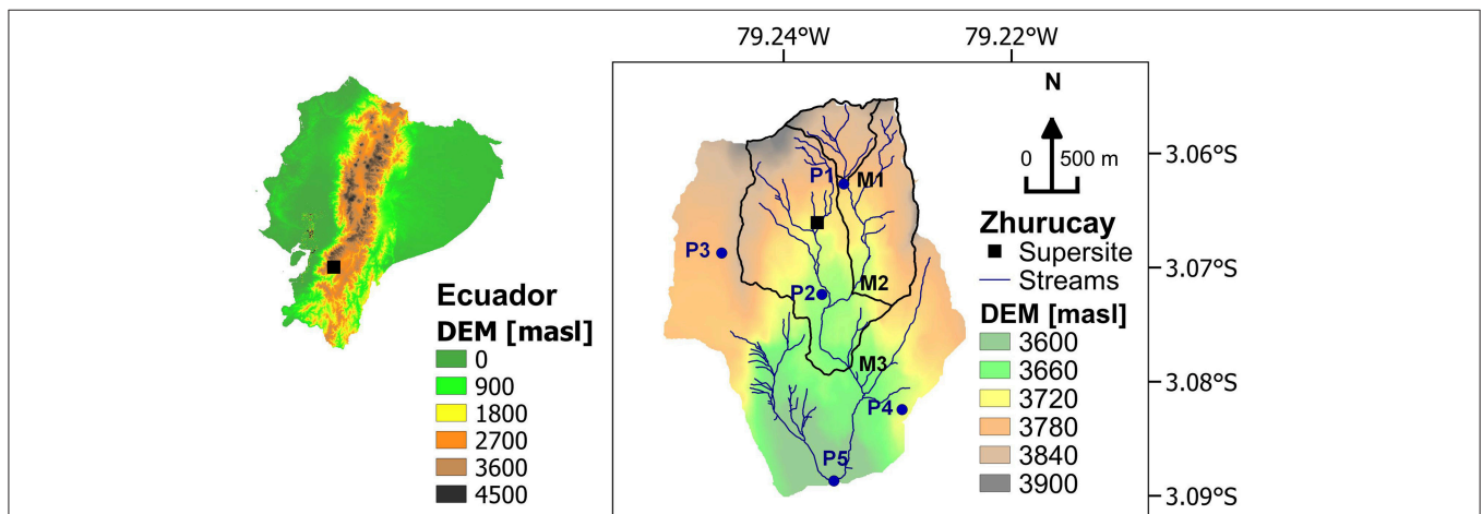
FIGURE 1 | Zhurucaj Ecohydrological Observatory located in Southern Ecuador. Three main microcatchments within the Zhurucaj Observatory are numbered from M1 to M3 and five rain gauges are numbered from P1 to P5.
