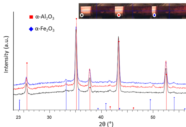
Figure 10. \mu -XRD results of the Fe-CMR p prepared by the precipitation of a Fe complex and calcined at 900 °C.
