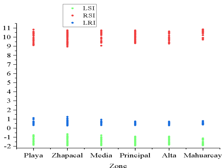
Figure 3. Variation of corrosion indexes in the different zones.
