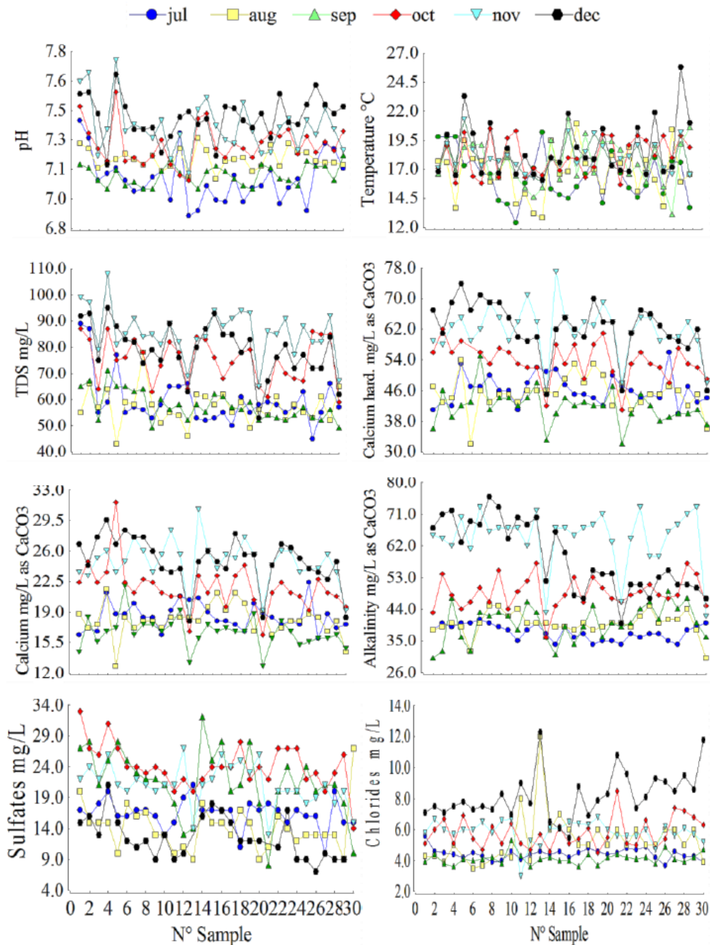
Figure 2. Variation of pH, temperature, TDS, calcium, alkalinity, sulfates and chlorides of drinking water in the distribution network sampling points.
