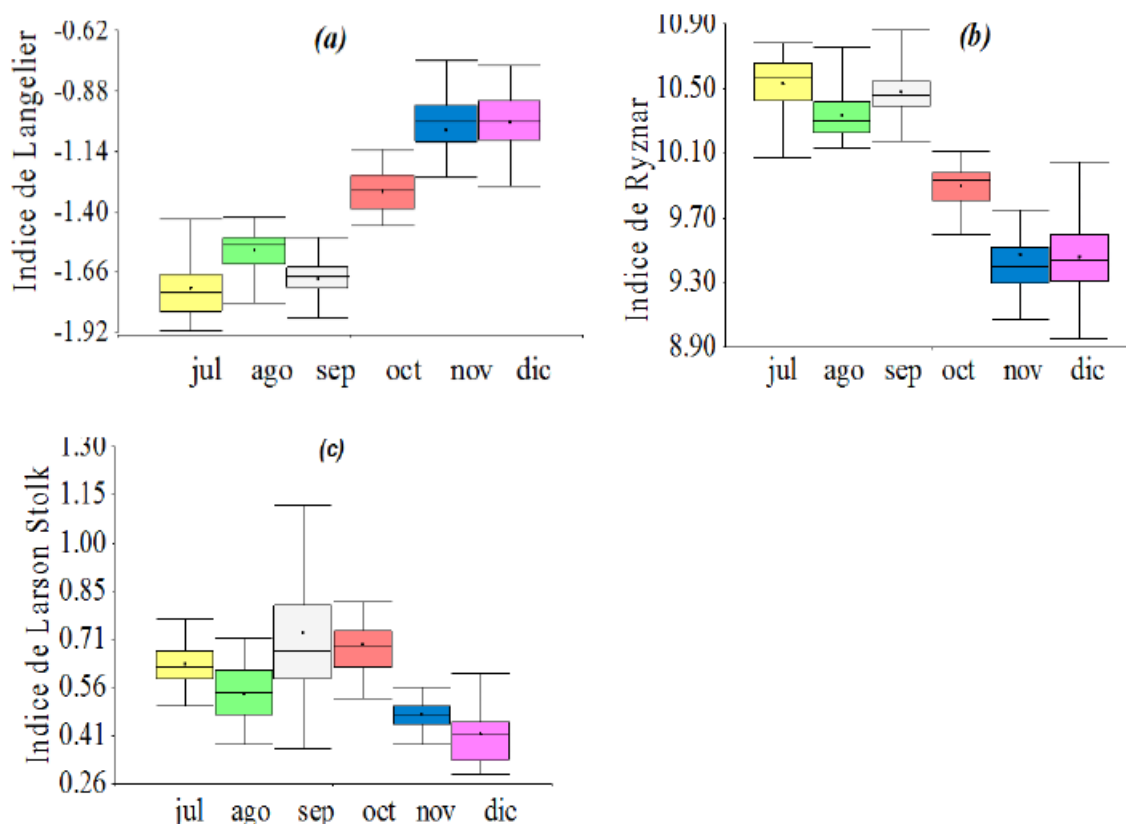
Figure 5. Variation of corrosion indexes over time. (a) Variation of LSI with months, (b) Variation of RSI with months, (c) Variation of LRI with months.
