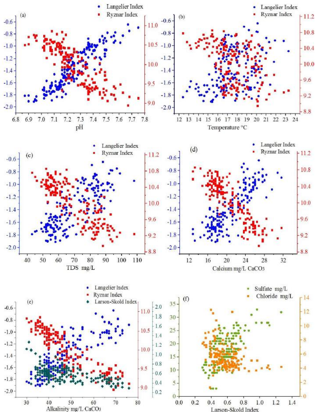
Figure 4. Variation of corrosion indexes with physical-chemical parameters. (a) pH relationship with LSI and RSI; (b) temperature relationship with LSI and RSI; (c) TDS relationship with LSI and RSI; (d) calcium relationship with LSI and RSI; (e) alkalinity relationship with LSI, RSI and LRI; (f) LRI relationship with sulfates and chlorides.
