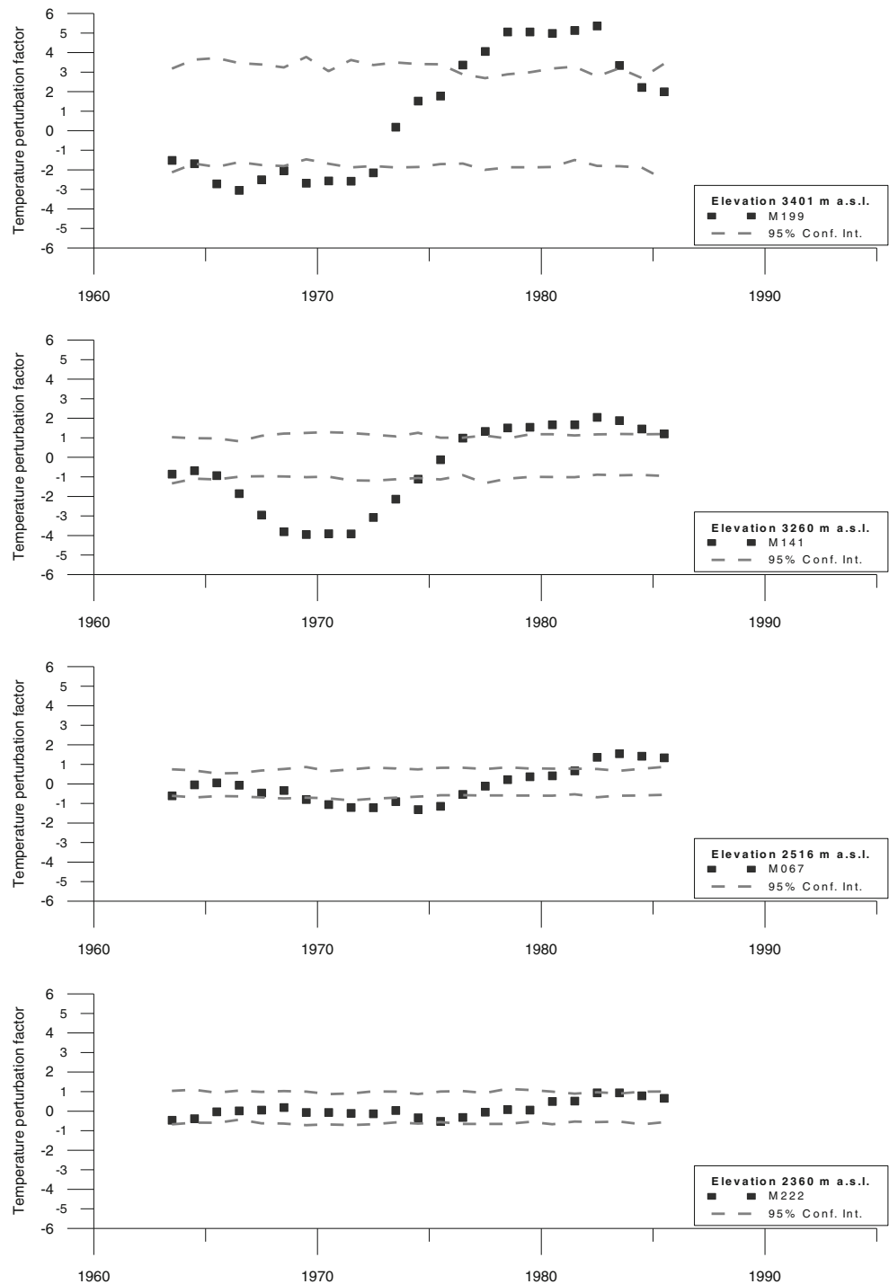
Fig. 2 Quantile perturbation analysis results for temperature and 95% confidence intervals on the perturbation factors: all seasons. All perturbation factors are in percent
