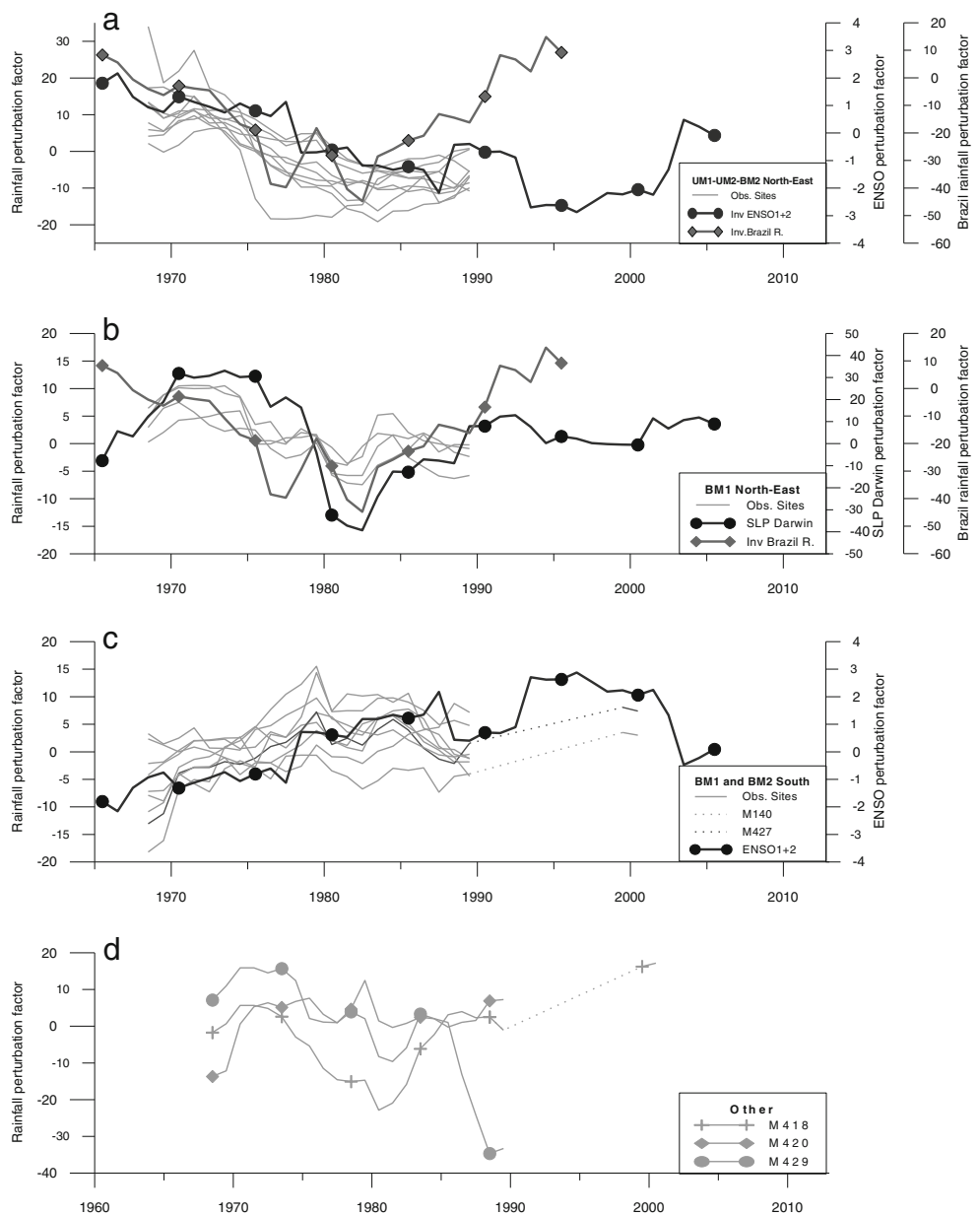
Fig. 4 Rainfall, ENSO, and large-scale climate quantile perturbation analysis results: all seasons. a UM1, UM2, and BM2 northeast aspect; b BM1 northeast; c BM1 and BM2 south aspect; and d other. All perturbation factors are in percent
