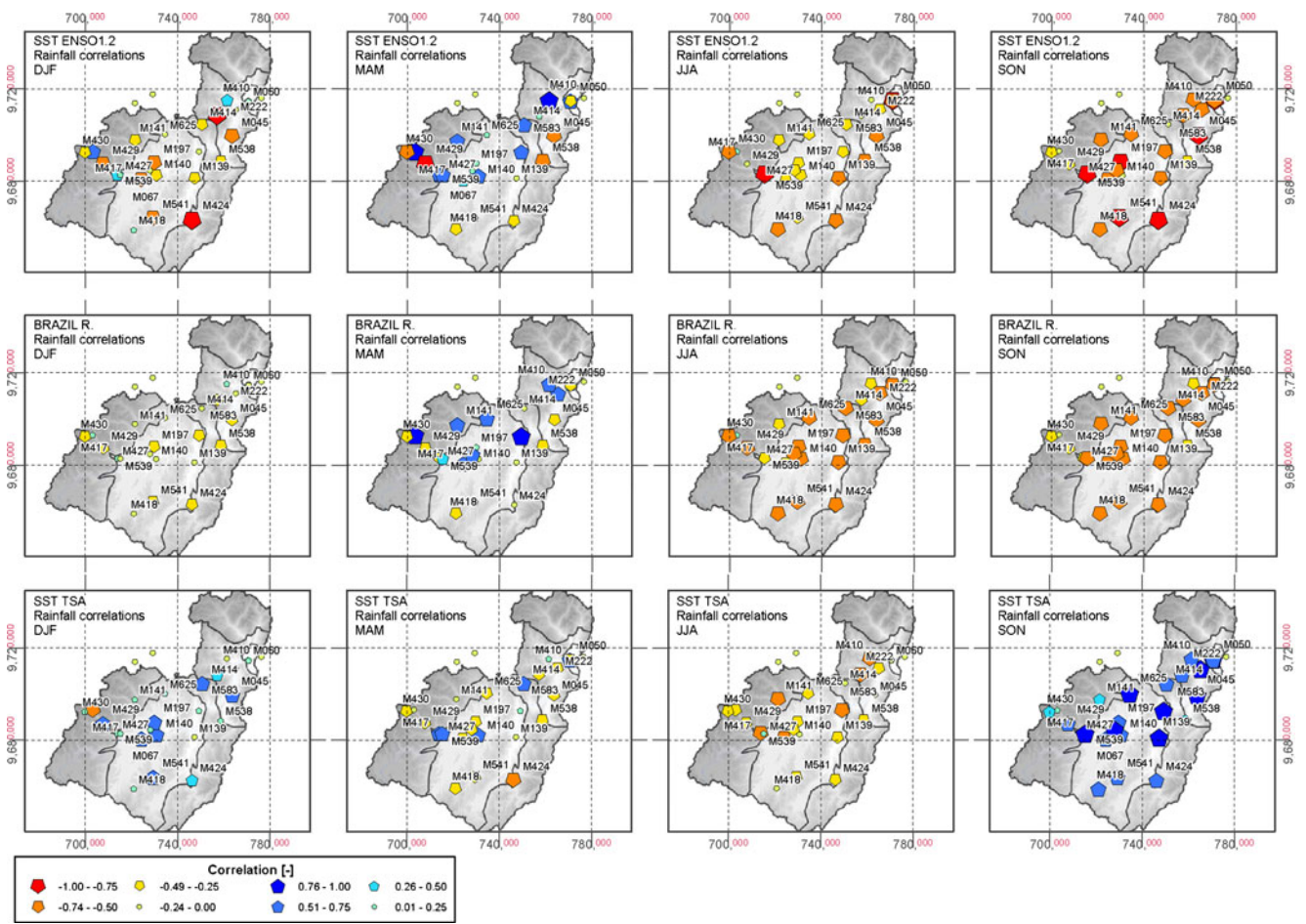
Fig. 7 Correlation between anomalies of observed sites and anomalies of different large-scale climate influences for rainfall in different seasons
