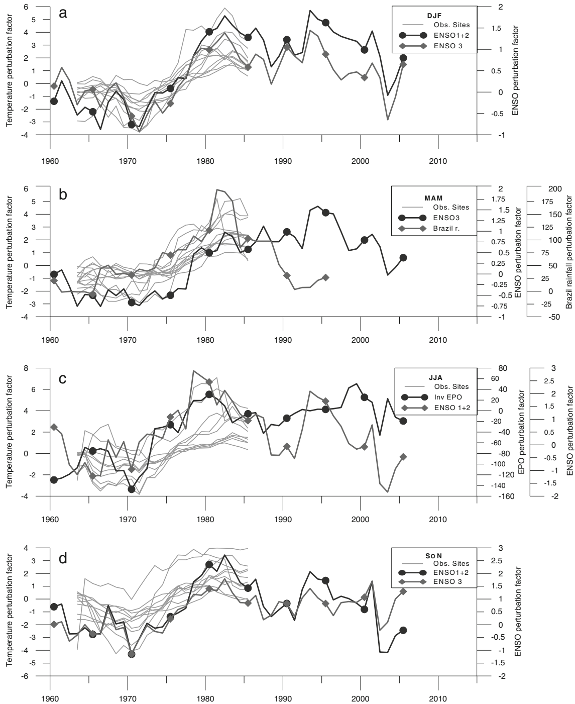
Fig. 6 Temperature and large-scale climate quantile perturbation analysis results for individual seasons. a DJF, b MAM, c JJA, and d . SON. All perturbation factors are in percent
