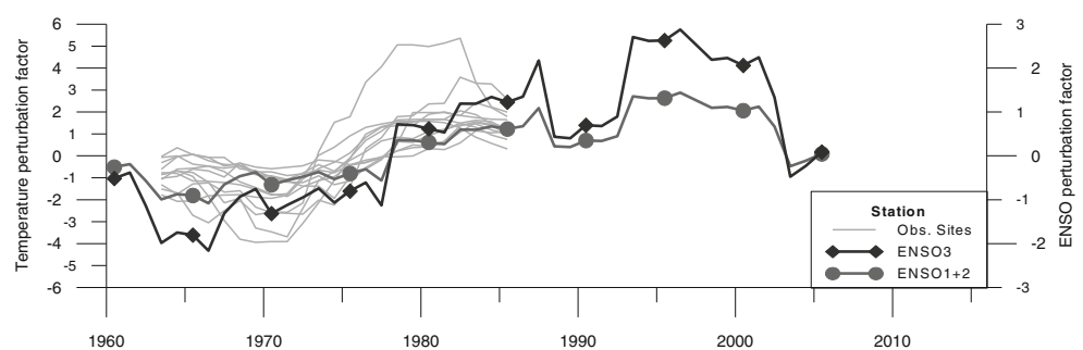
Fig. 3 Temperature and ENSO SST quantile perturbation analysis results: all seasons. All perturbation factors are in percent
